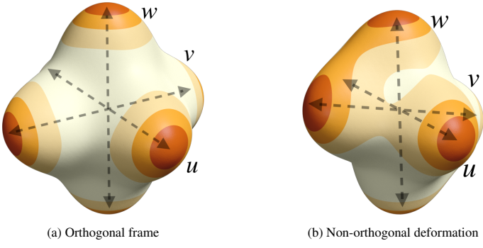
Figure 8: 3-Direction sets \{u, -u, v, -v, w, -w\} represented by spherical polynomials of degree 4.
