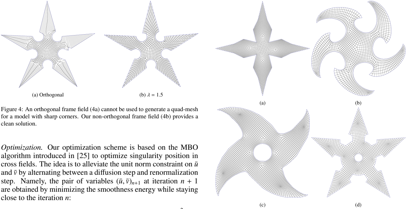
Figure 5: Our method is able generate nicely shaped quad-meshes by adjusting the parameter \lambda = 1.5 .
