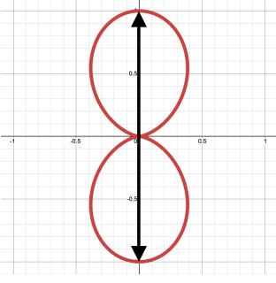
Figure 1: A unique direction (black arrows) represented by a polar (left) and spherical (right) polynomial of degree 2. The value of the polynomial at each point of the circle is represented as a variation of the radius in polar coordinates.
