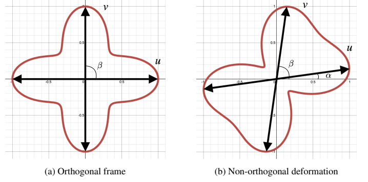
Figure 2: A 2-Direction set \{u, -u, v, -v\} (black arrows) represented by a polar polynomial of degree four.
